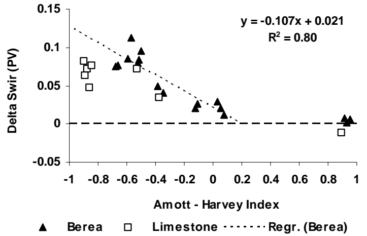
Fig. 12 Magnitude of S_{wir} underestimation versus Amott-Harvey index
