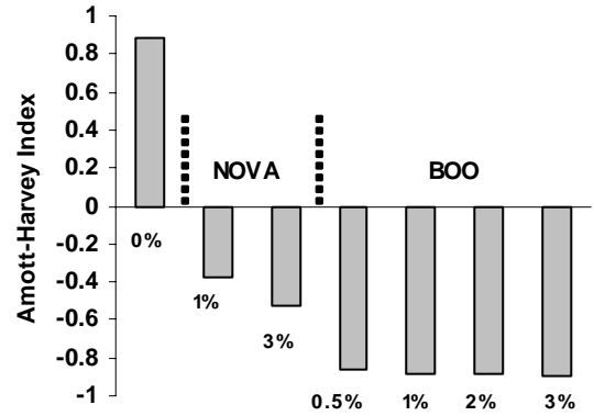
Fig. 2 Amott-Harvey indices of limestone cores after flushing
