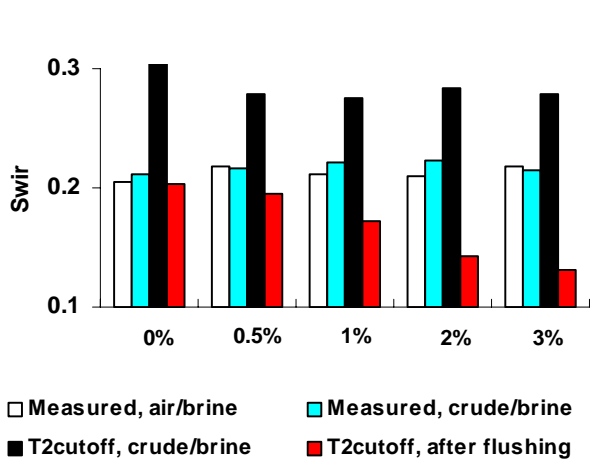
Fig. 8 S_{wir} measured by weighing and estimated from T_{2, cutoff} of 33 ms (Berea cores, OBM surfactant system: BOO)
