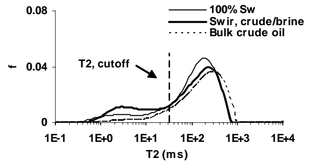
Fig. 6 Interfere of relaxation time of bulk crude oil with that of irreducible water (Berea core B30).
