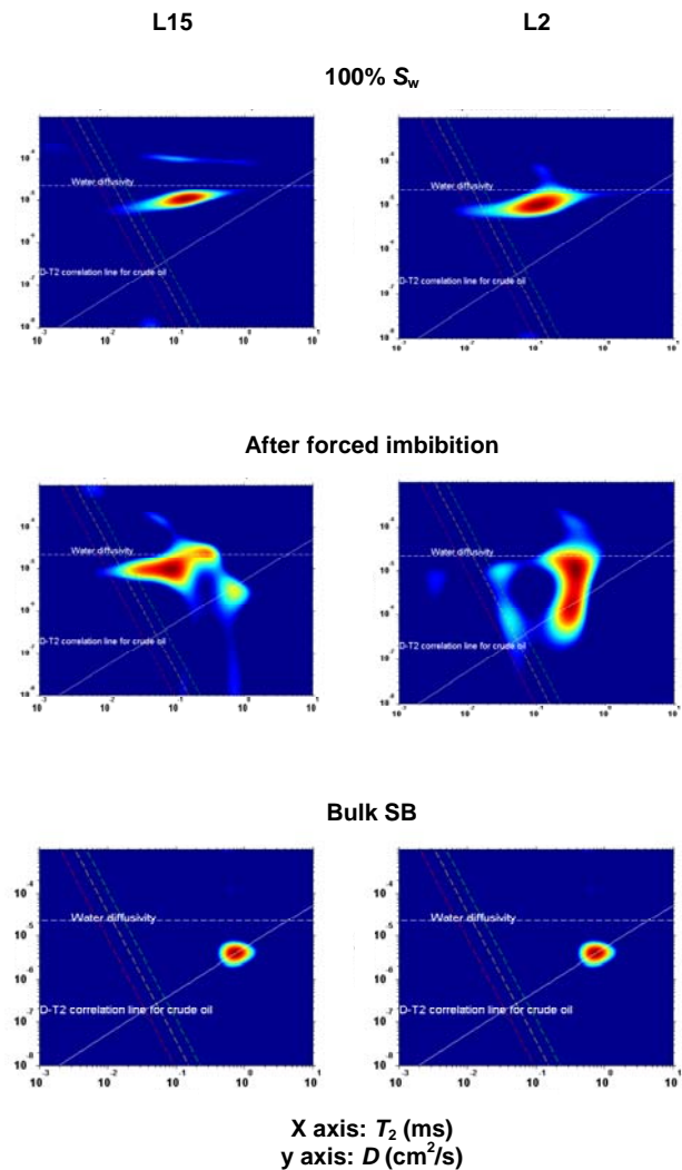
Fig. 3 Diffusion editing maps of 100% S_w , after forced imbibition and bulk SB for Limestone L15 (left, water-wet after flushing) and L2 (right, oil-wet after flushing)
