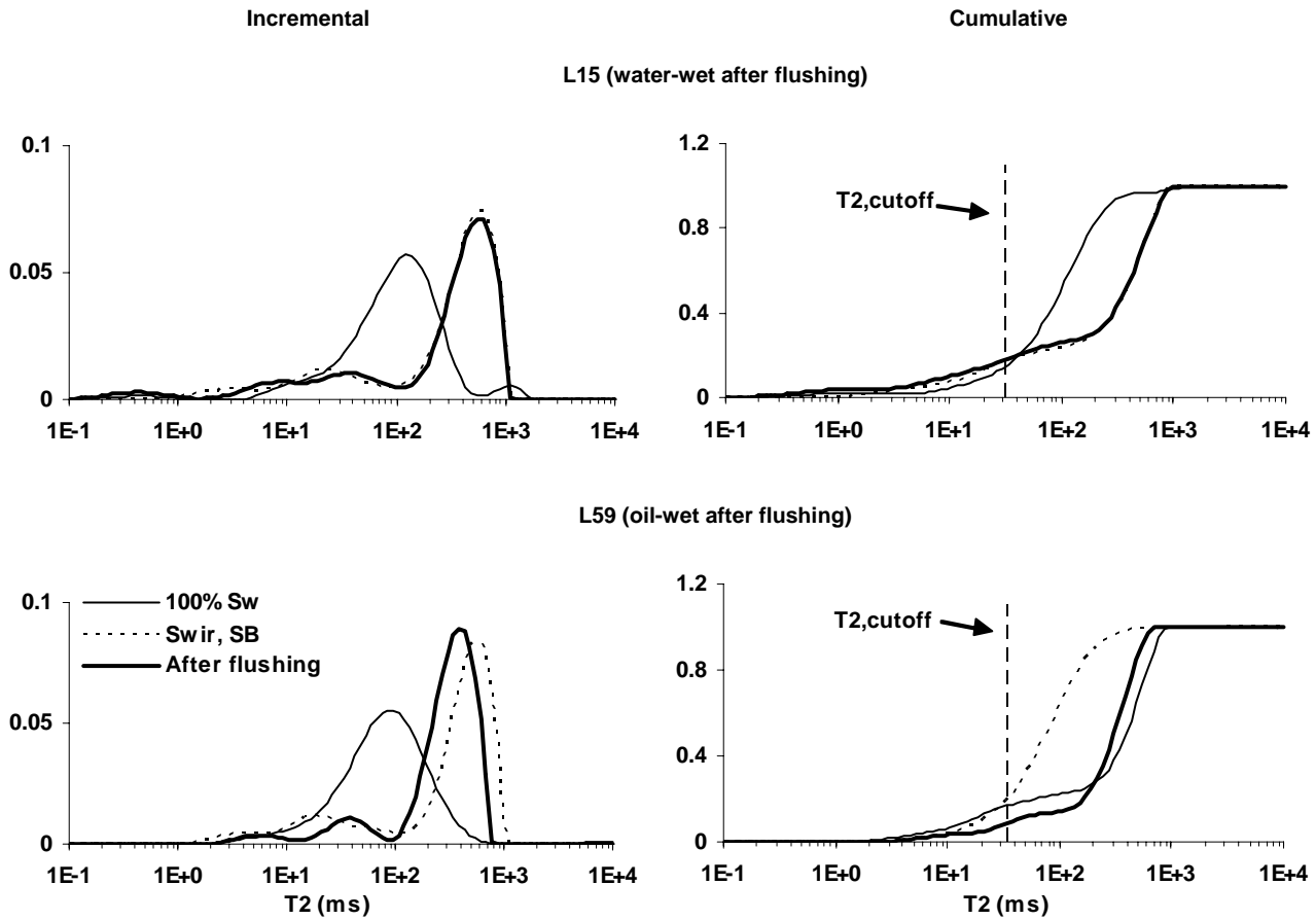
Fig. 7 Incremental and cumulative T_2 distributions for limestone L15 and L59 at 100% S_w , S_{wir} with SB and after flushing.
