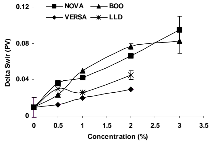
Fig. 9 Magnitude of S_{wir} underestimation with respect to the OBM surfactants concentration in the flushing fluid (Berea cores).
