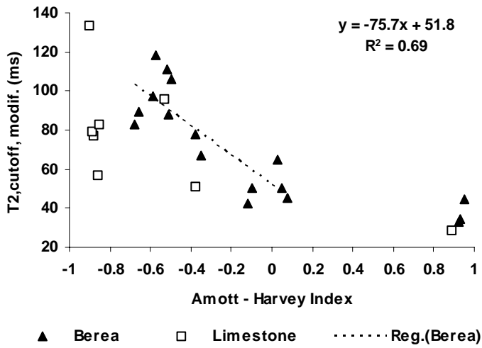
Fig. 16 Modification of T_{2,cutoff} versus Amott-Harvey wettability index.
