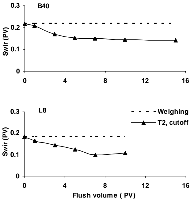
Fig. 11 Effects of flush volume on S_{wir} underestimation for Berea B40 (top) and limestone L8 (bottom)
