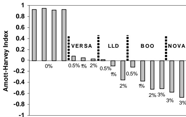
Fig. 1 Amott-Harvey indices of Berea cores after flushing
