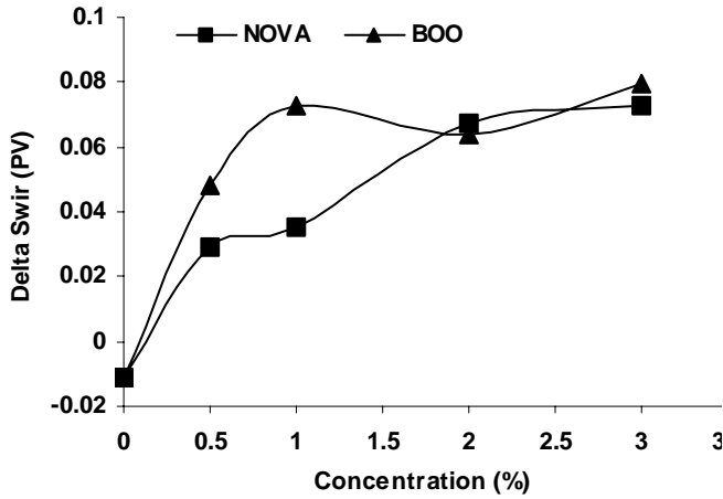
Fig. 10 Magnitude of S_{wir} underestimation with respect to the OBM surfactants concentration in the flushing fluid (limestone cores).
