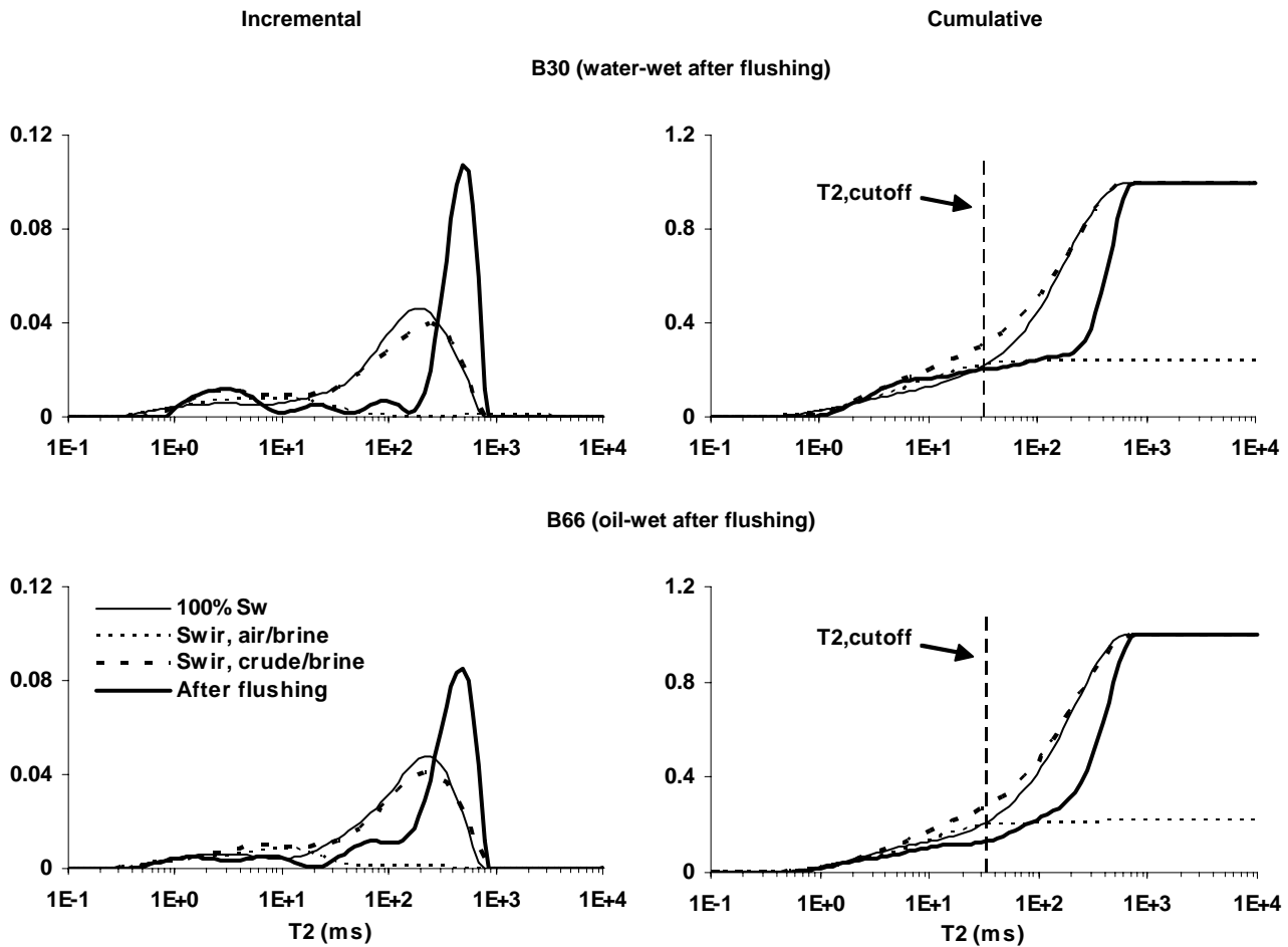
Fig. 5 Incremental and cumulative T_2 distributions for Berea B30 and B66 at 100% S_w , S_{wir} with air, S_{wir} with crude oil and after flushing.
