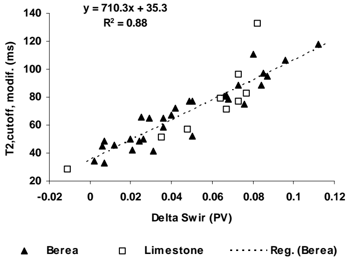
Fig. 15 Modification of T_{2,cutoff} versus magnitude of S_{wir} underestimation.
