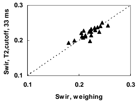
Fig. 4 Cross-plot of S_{wir} by weighing and from T_{2,cutoff} of 33 ms for 100% S_w of Berea cores.
