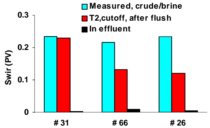
Fig. 13 Karl-Fisher analysis of water amount in the flushing effluents.
