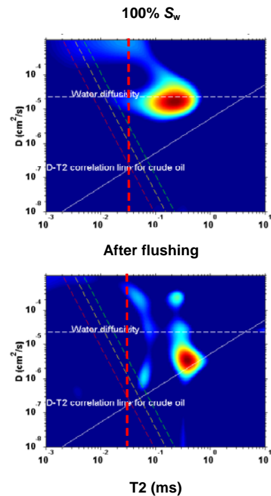
Fig. 14 Diffusion editing maps of 100% S_w and after flushing for Berea core B77 (red dashed line: T_{2,cutoff} of 33 ms).
