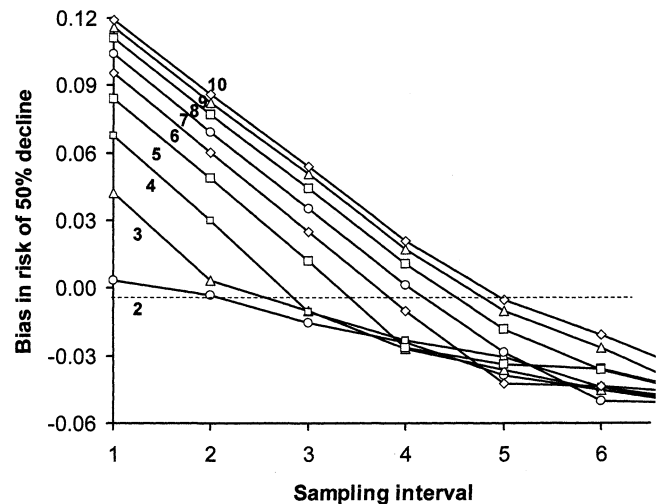
Figure 1. Bias in risk of 50% decline for scalar models relative to matrix-based models under different generation times (from 2 to 10 years as indicated for each curve) and as a function of the census period. The nine structured models have the same finite rate of increase (eigenvalue = 1.0), annual survival rate (0.5), and variation (CV for fecundity = 10%; CV for survival = 5%) but varying generation times.
