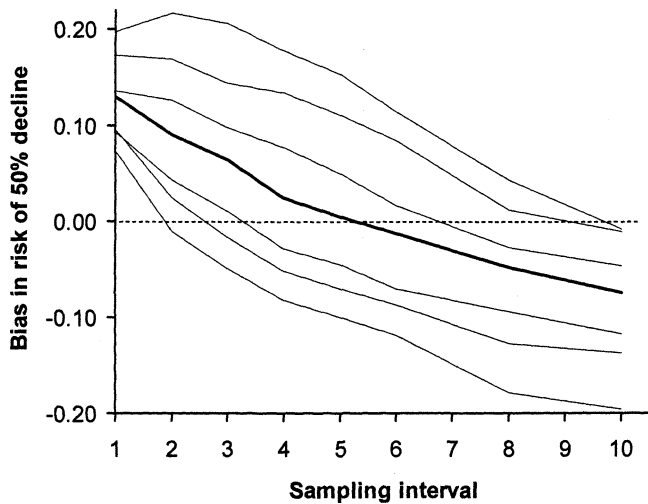
Figure 2. Effect of initial age structure on the bias in the prediction of scalar models. Bias and sampling interval are as in Fig. 1. All age-structured models had a generation time of 10 years. Initial age structure was varied by changing the proportion of individuals in the breeding (two oldest) age classes from 0.16% (lowest curve) to 0.64% (highest curve) in increments of 0.08%. At the stable age distribution, the percentage in breeding age classes is about 0.4% (the middle curve).
