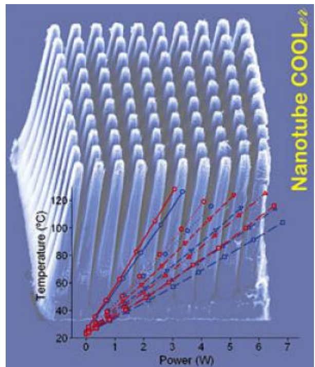
Red graph lines show the temperature of a bare chip as increased power is applied, while blue lines show the reduced temperatures of a chip equipped with a carbon nanotube cooling structure (pictured in the background). Solid and dashed lines represent experimental and computational results, respectively. Both natural and forced convection conditions are noted. (Credit: Rensselaer/Robert Vajtai)
