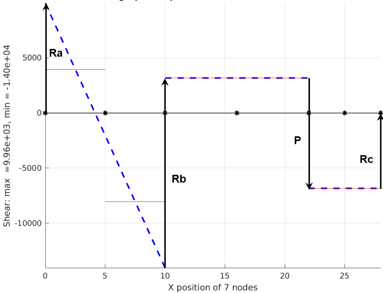
Shear graph for quintic and cubic (red) C1 elements
